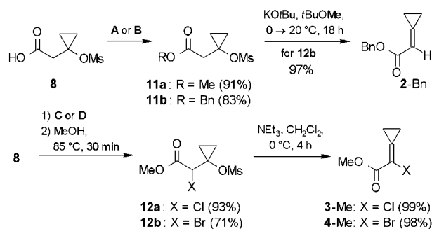
Scheme 4. Transformation of 8 to cyclopropylideneacetates 2-4 . A : MeOH, cat. H 2 SO 4 , 20 °C, 12 h; B : BnOH, cat. p TsOH, toluene, 60 °C, 6 h; C : SOCl 2 , NCS, cat. conc. HCl, 1,2-DCE, 85 °C, 15 h; D : SOCl 2 , NBS, cat. conc. HBr, 1,2-DCE, 85 °C, 15 h.
