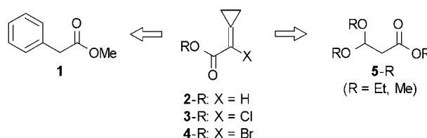
Scheme 1. Retrosynthetic considerations concerning cyclopropylideneacetates 2–4 .
