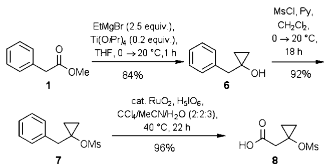
Scheme 2. Preparation of 2-(1'-mesyloxycyclopropyl)acetic acid ( 8 ) from methyl phenylacetate ( 1 ).
