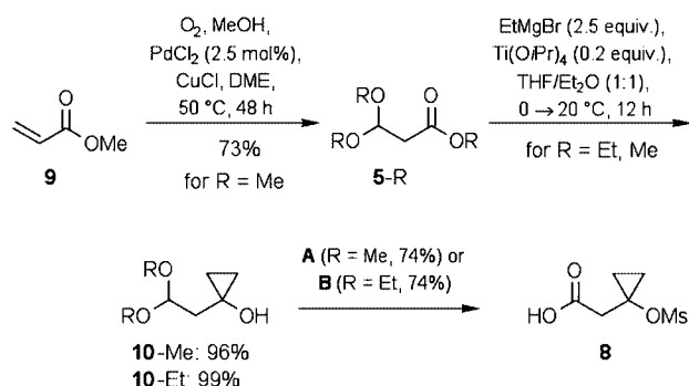
Scheme 3. Alternative preparation of 2-(1'-hydroxycyclopropyl)acetic acid ( 8 ) from methyl acrylate ( 9 ) or ethyl 3,3-diethoxypropionate ( 5-Et ). A : 1) MsCl, Py, CH 2 Cl 2 , 20 °C, 15 h, 2) cat. conc. HCl, H 2 O 2 , THF/H 2 O (2:1), 60 °C, 8 h; B : 1) MsCl, cat. DMAP, NEt 3 , CH 2 Cl 2 , 20 °C, 4 h, 2) Oxone, THF/H 2 O (1:2), 20 °C, 8 h.
